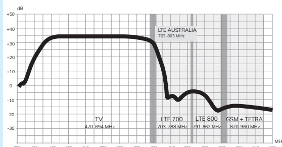
Gain curve
