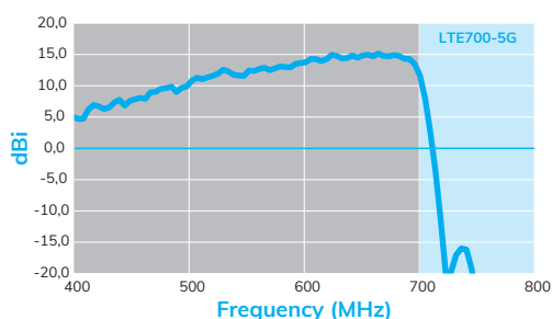
Gain curve
